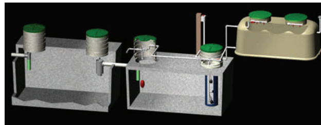
Typical Residential Advanced Treatment System Layout
