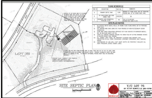
Residential Septic System Site Plan
