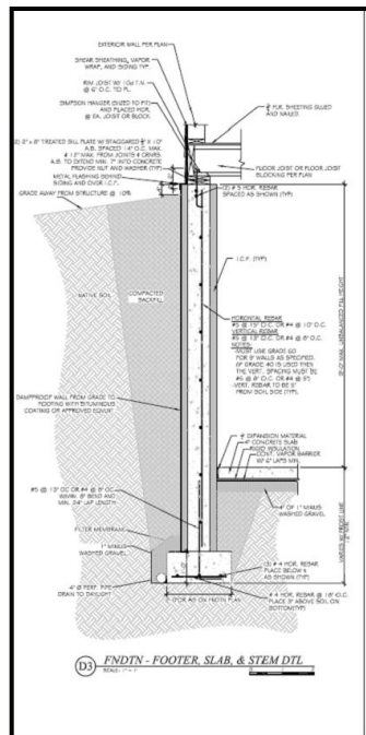
Basement Wall Detail
