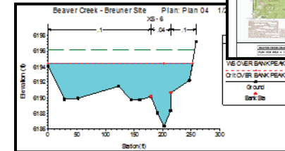
HEC-RAS Overbank Flow Simulation
