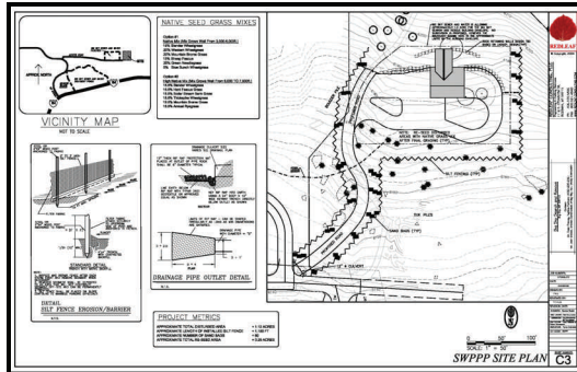
Storm Water Pollution Prevention Plan Big Sky Search and Rescue Building
